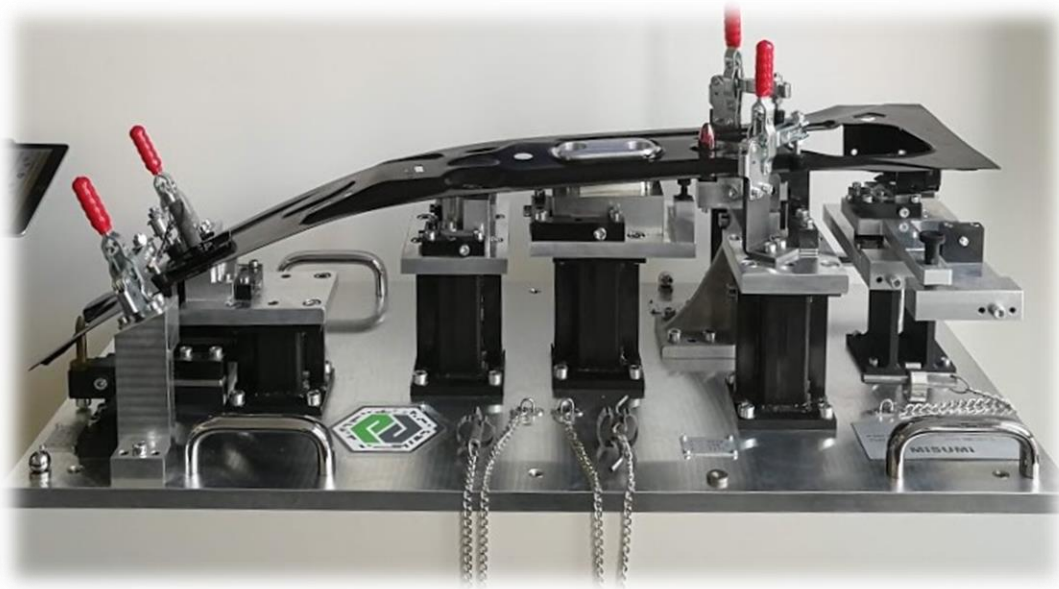
Demo Machine from customer Misumi (It's a B-pillar testing machine)
